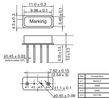
F-11 Type
