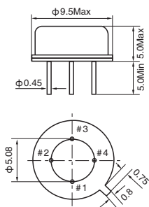
TO39B Type
