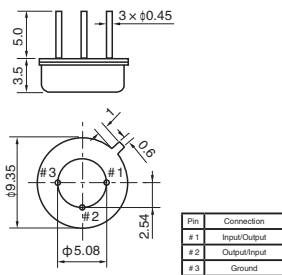
TO-39 Type
