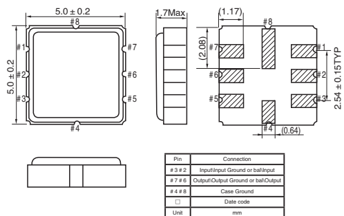
SM-55 Type
