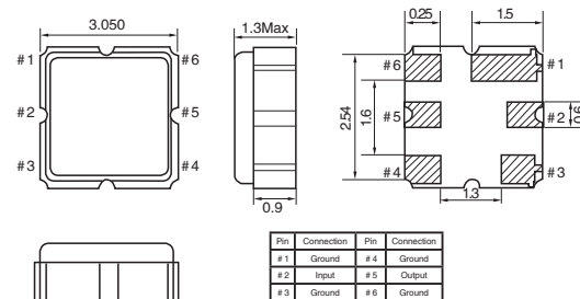
SM-33 Type
