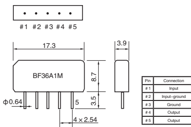
SIP5K Type
